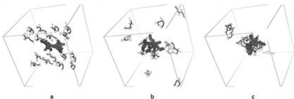
Figure 2. Snapshots of the dendrimer and Semax peptides at different time moments: t = 0 (a), t = 20 ns (b), t = 160 ns (c).
